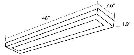
Wall Mount Dimensions
