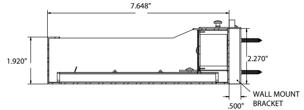
Wall Mount Dimensions
